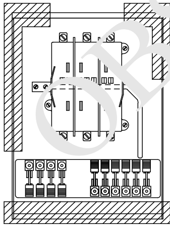
ZS3-20 FOR 4 WIRE SERVICE 13 TERMINAL CT METER SOCKET
