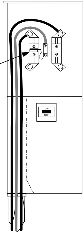
Network, CL200, 3W, 120/208V
