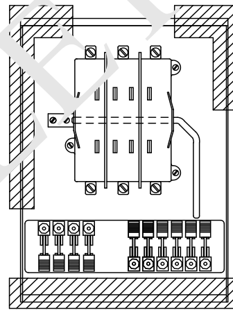
ZS3-20-5S FOR 3 WIRE SERVICE 8 TERMINAL CT METER SOCKET
